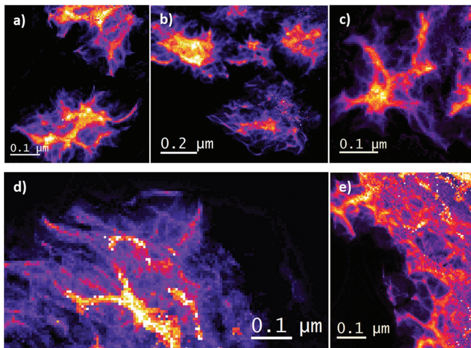
Figure 5. Examples of quantitative silicon phase maps for pH 4 and pH 6 samples a–c) after 30 cycles and d,e) after 100 cycles. Solely the silicon contribution is presented here. Instead of a linear red gradient used in all previous phase maps, the color scale was chosen as “black body extended” in order to better visualize the filaments and the “hairy” nature of the peripheral silicon around the cores.
