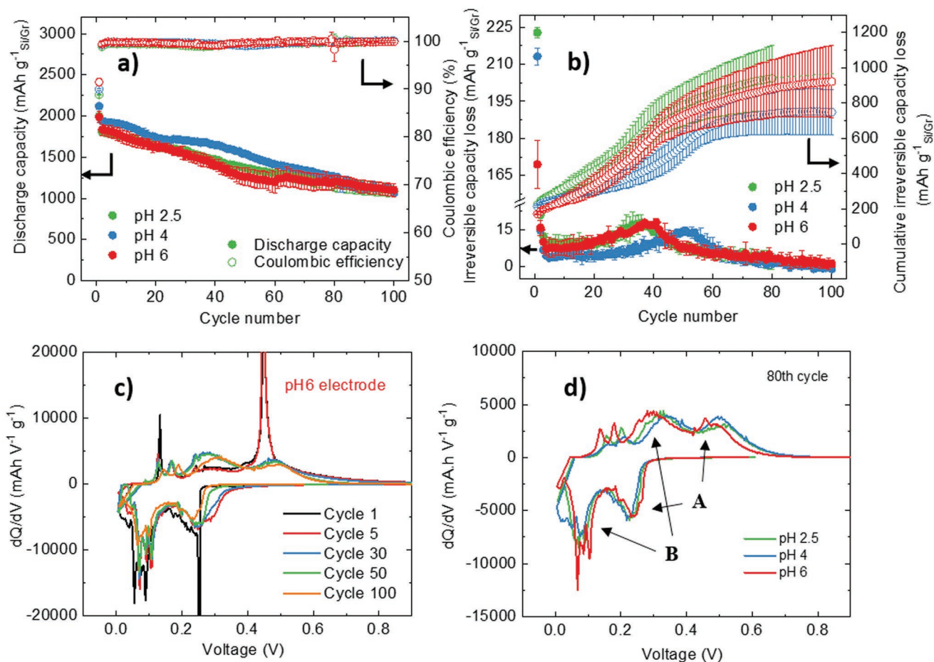
Figure 1. Half-cell electrochemical cycling of Si/Gr electrode prepared at pH 2.5, 4 and 6 (coin cells). a) Discharge capacity evolution; b) irreversible and cumulative capacity loss versus cycle number; c) incremental capacity–voltage curve for pH 6 electrode during the electrochemical cycling, similar behaviors were observed for pH 2.5 and 4 at different cycles, except for 100th cycle; d) comparison of incremental capacity–voltage curve for pH 2.5, 4 and 6 at 80th cycle.
