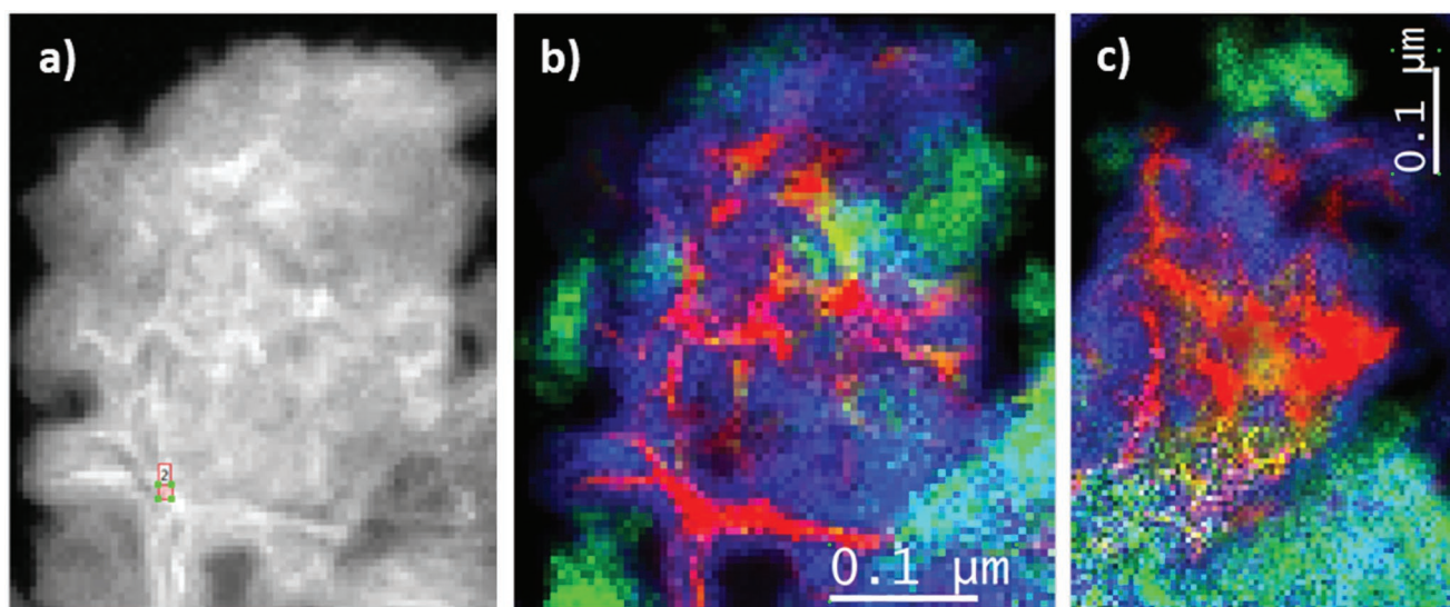
Figure 4. Example of a quantitative mapping on the cycle 100 pH 4 sample: a) STEM-HAADF image on silicon flake; b) corresponding quantitative map of the repartition of the three phases (no graphite in this region). c) Other quantitative map example of the same electrode. In both b) and c) the mixing of PAALi and LiF is visible at the bottom right where the turquoise color results from the blue (PAALi) and green (LiF) superposition.
