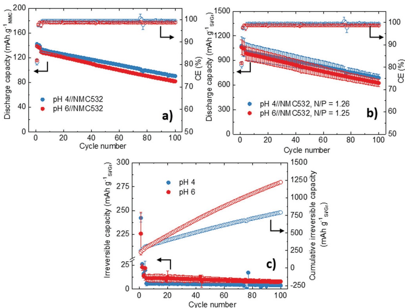
Figure 7. Full cell electrochemical cycling of Si/Gr negative electrodes prepared at pH 4 and 6 (coin cells) with NMC532 positive electrode. a) Discharge capacity in mAh per g of NMC versus cycle number; b) discharge capacity in mAh per g of Si/Gr versus cycle number; c) irreversible and cumulative capacity loss versus cycle number.
