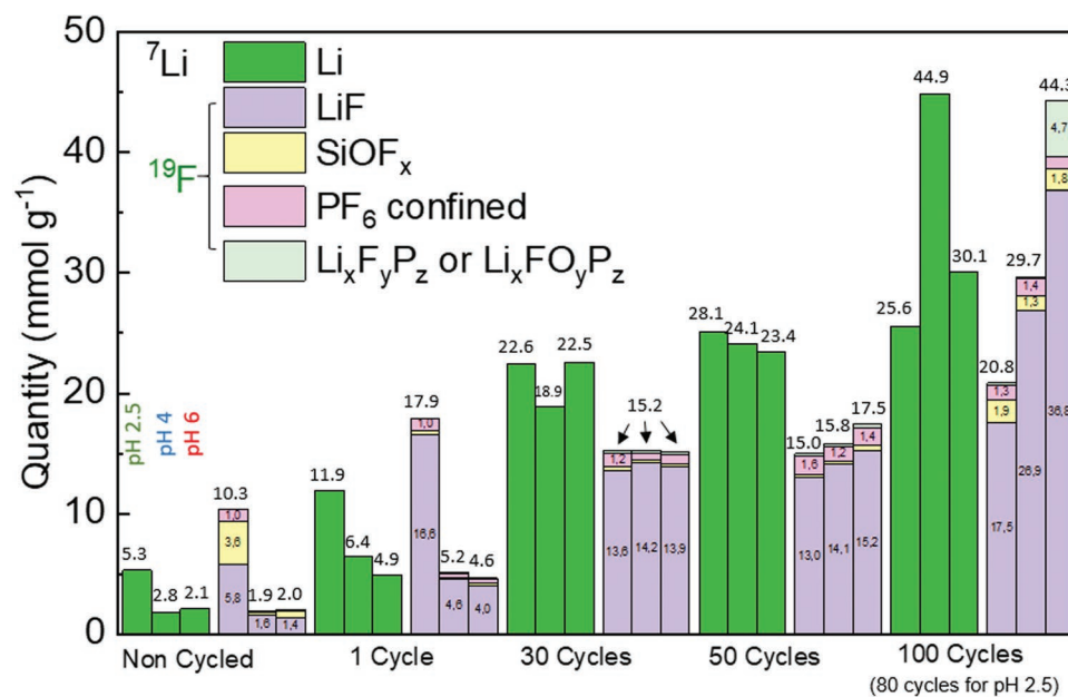
Figure 6. MAS NMR {}^7\text{Li} and {}^{19}\text{F} quantitative results of electrodes adjusted at pH 2.5, 4 and 6 non cycled and after the 1st, 30th, 50th, and 80th (for pH 2.5) or 100th cycle.
