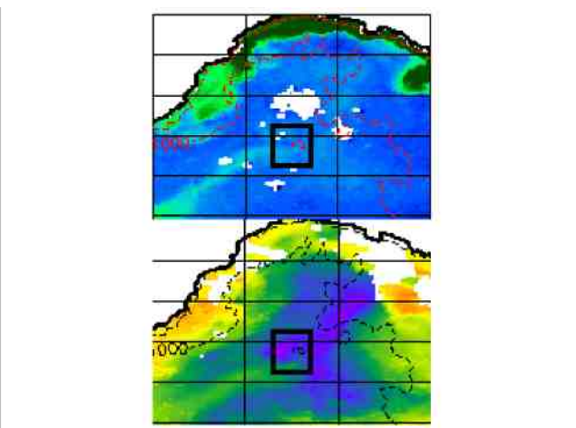
Surface chlorophyll (top) and temperature (bottom) of the 6 November 2016. (Data provided by CMEMS).
