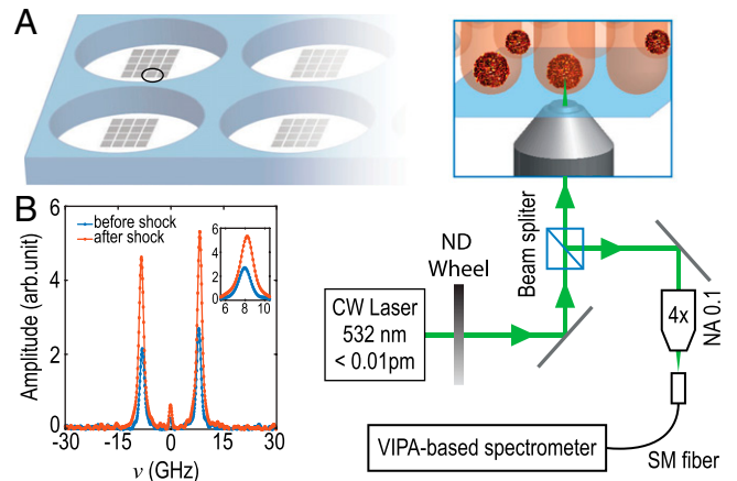
Fig. 2. (A) Schematic of microstructured wells for MCS; the virtually imaged phase array (VIPA)-based Brillouin spectrometer is coupled with a microscope. (B) Typical spectrum obtained at the center of an MCS before and after the shock. (Inset) Zoomed-in view of the anti-Stokes shift. SM, single mode. NA, numerical aperture; ND, neutral density; CW, continuous wave.
