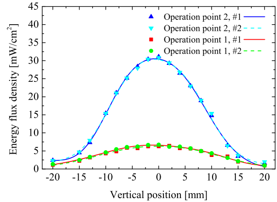
Fig. 9. Energy flux density vs. vertical position for the RIT- \mu X running at operation point 1 and 2 measured with the active thermal probe. The symbols represent the experimental data, the solid lines give cubic spline interpolations as a guide to the eye. There are two measurements for each operation point.
