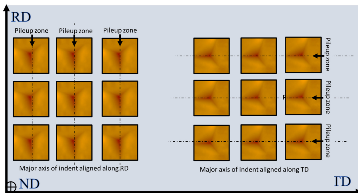
Figure 3. Schematic showing the nanoindentation performed along the RD and TD of a Cu(16)/Nb(16) ARB nanolaminate by aligning the major axis of the Berkovich tip along the TD and RD obtained using SPM. The height profiles were then plotted along the major axis of the indentations (represented as dashed lines) for RD and TD as shown in Section 3.3, and later used to measure the pile-up along these directions.
