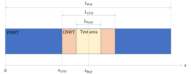
FIGURE 1: TWO-DIMENSIONAL SIMULATION DOMAIN. THE TEST AREA IS EMBEDDED IN THE CNWT DOMAIN, WHICH IS EMBEDDED IN THE PNWT DOMAIN. POSSIBLE OVERLAY ZONES FOR COUPLING ARE NOT REPRESENTED.
