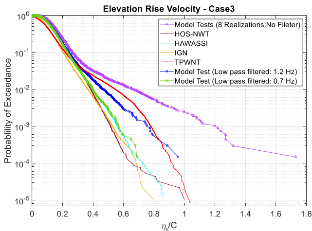
FIGURE 11: ENSEMBLE PROBABILITY DISTRIBUTION OF WAVE-ELEVATION RISE VELOCITY FOR CASE3
