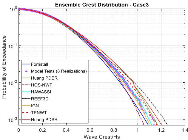
(b) Ensemble crest distribution - probability up to 7 \times 10^{-4}
