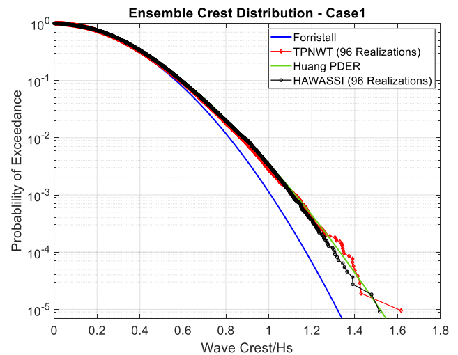
FIGURE 6: ENSEMBLE PROBABILITY DISTRIBUTION OF CREST HEIGHT FOR CASE1
