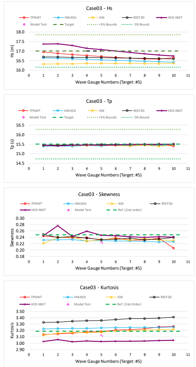
FIGURE 9: HS, TP, SKEWNESS AND KURTOSIS AT WAVE GAUGES (WG1 – WG10) FOR CASE3
