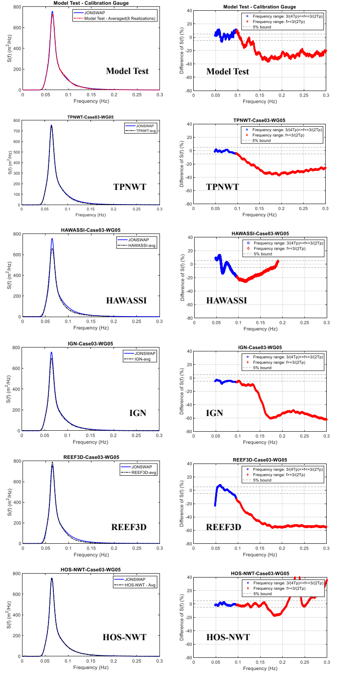
FIGURE 8: WAVE SPECTRUM (LEFT) AND RATIO BETWEEN SIMULATED AND TARGET SPECTRUM (RIGHT) FOR CASE 3
