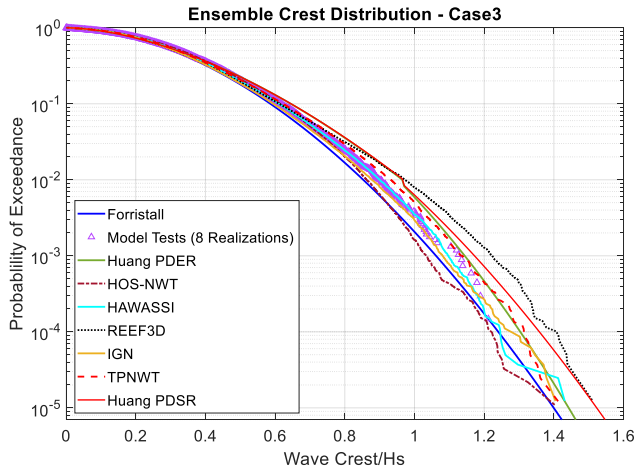
(a) Comparison of ensemble crest distribution
