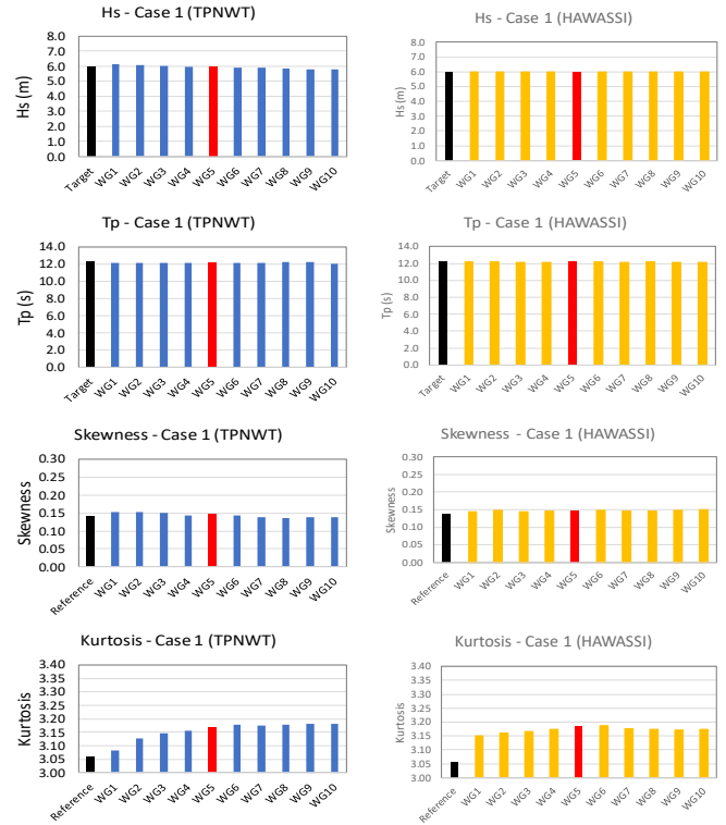
FIGURE 5: H_s , T_p , SKEWNESS AND KURTOSIS AT WAVE GAUGES (WG1 – WG10) FOR CASE1
