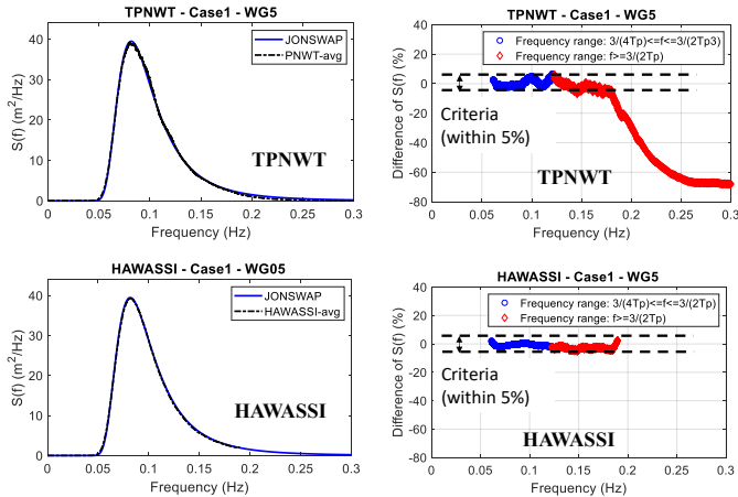
FIGURE 4: WAVE SPECTRUM (LEFT) AND RATIO BETWEEN SIMULATED AND TARGET SPECTRUM (RIGHT) FOR CASE1
