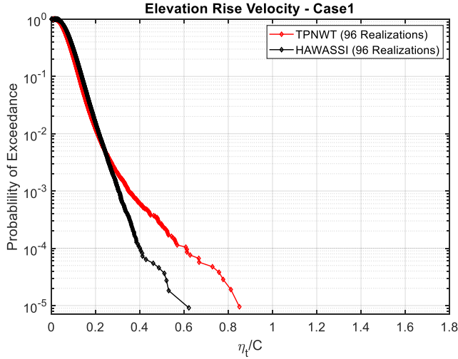
FIGURE 7: ENSEMBLE PROBABILITY DISTRIBUTION OF WAVE-ELEVATION RISE VELOCITY FOR CASE 1
