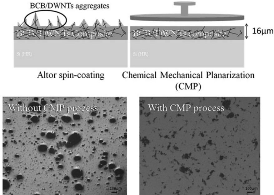
Fig. 2. Polishing process and optical microscope images of BCB/DWNT composite (0.127 wt%): (a) before CMP, and (b) after CMP.
