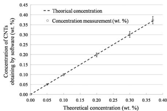
Fig. 4. Theoretical concentrations versus measured concentrations with Image J software.
