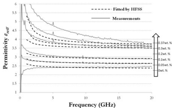
Fig. 6. Permittivity measurement (down stroke) and simulate (dotted line) for 0, 0.05, 0.1, 0.2, 0.3, and 0.37 wt% of CNT concentration.
