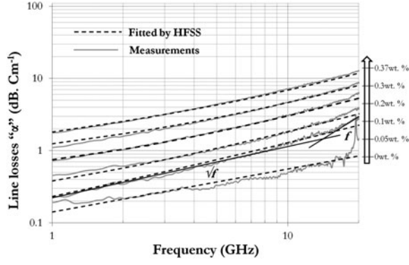
Fig. 5. Line losses measurement (solid) and simulate (dotted line) for 0, 0.05, 0.1, 0.2, 0.3, and 0.37 wt% of CNT concentration.
