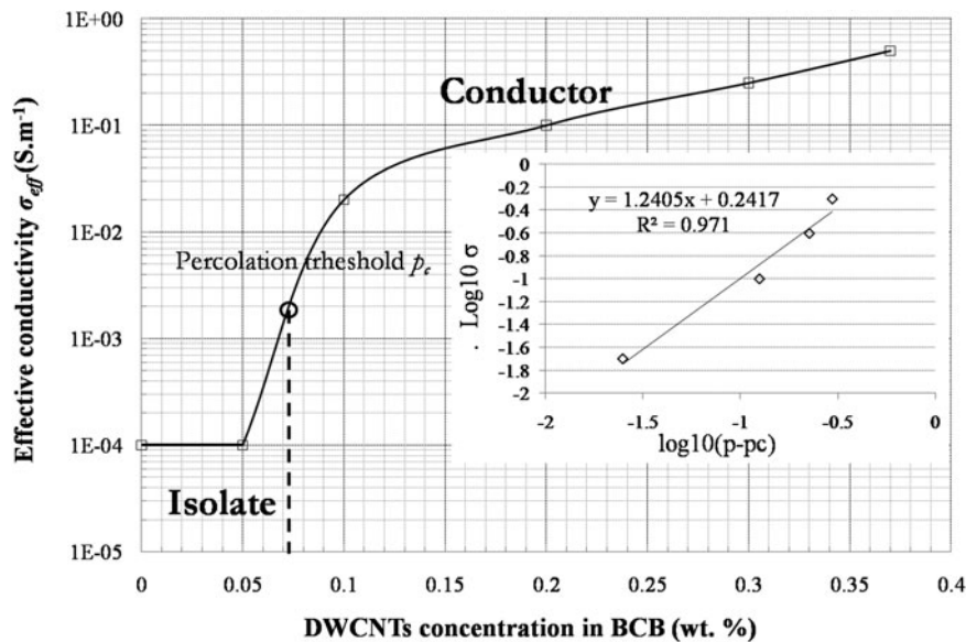
Fig. 8. Effective conductivity dependence on the CNT (in linear scale and \log_{10} - \log_{10} scale).
