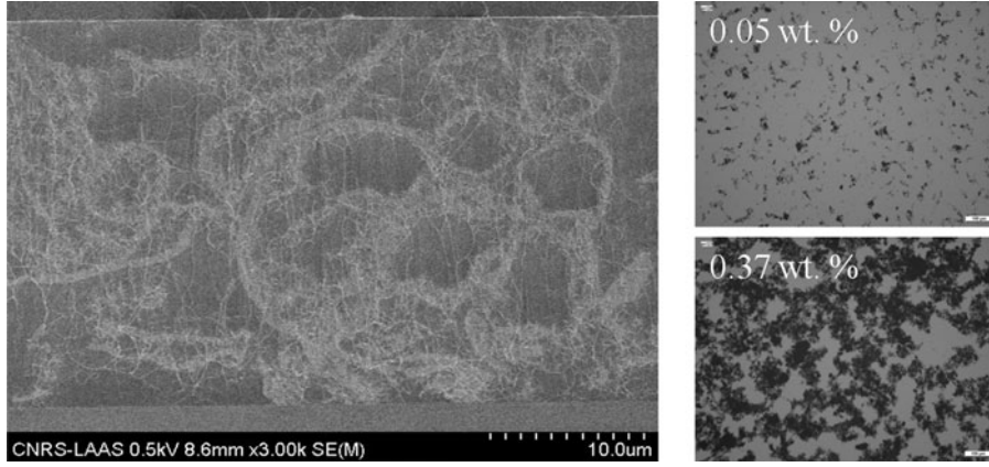
Fig. 1. SEM cross-sectional views of BCB/DWNT composites and optical microscope images of CNT-BCB composites at 0.05 and 0.37 wt%.
