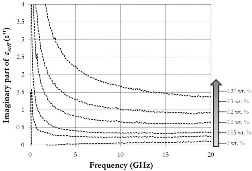
Fig. 7. The imaginary part of \epsilon_{eff} measurement for 0, 0.05, 0.1, 0.2, 0.3, and 0.37 wt% of CNT concentration.
