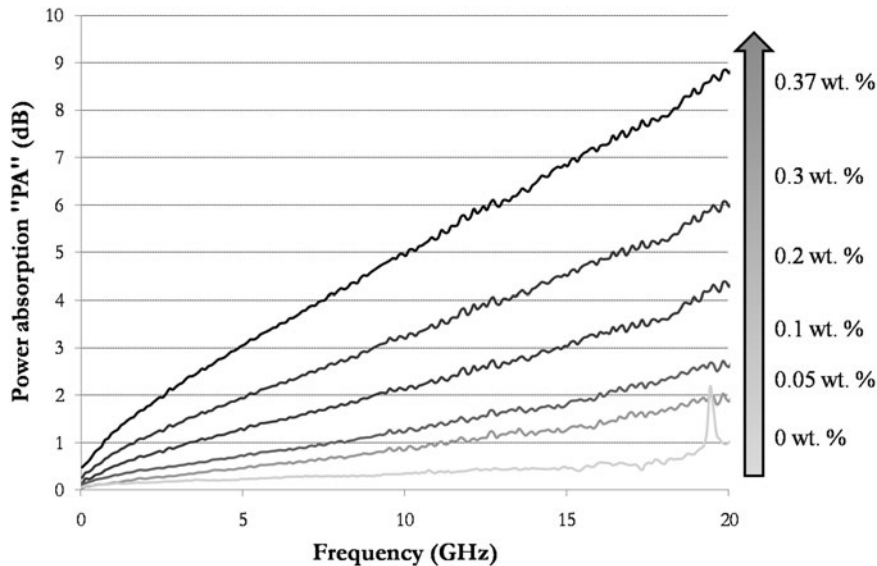
Fig. 9. PA for BCB/CNT containing 0, 0.05, 0.2, 0.3, and 0.37 wt% of inclusion.
