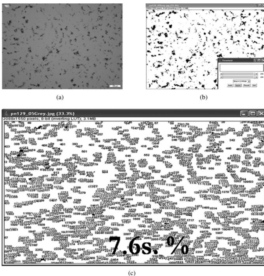
Fig. 3. Concentration characterization of CNT-BCB composites of 0.05 wt%: (a) monochrome optical microscope image, (b) tuning of threshold contrast (black point), and (c) particle analysis results in surface concentration (% s).
