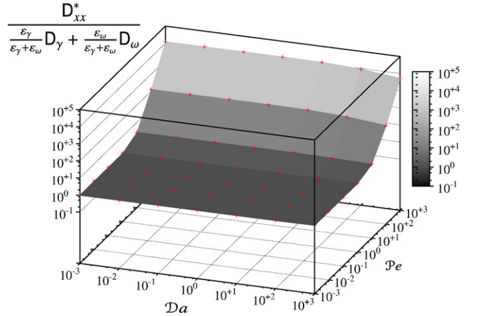
Fig. 5. Normalized longitudinal dispersion of the non-equilibrium model as a function of \mathcal{P}e and \mathcal{D}a numbers.
