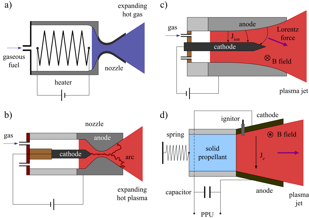
Figure 3. Schematic of electrothermal and electromagnetic thrusters: a) resistojet, b) arcjet thruster, c) self-field MPD thruster and d) ablative PPT.
