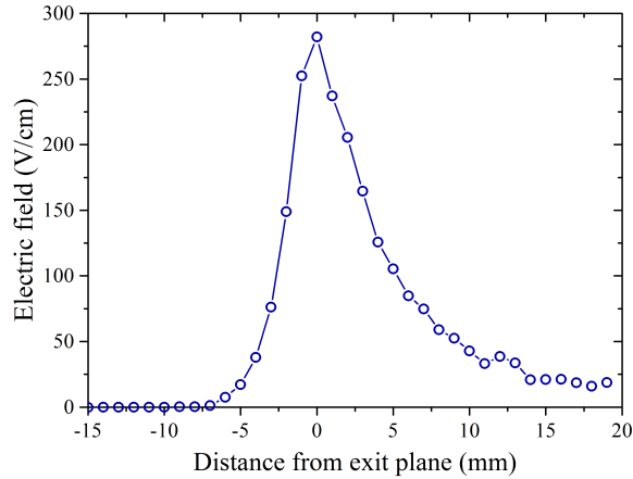
Figure 7. Electric field distribution along the channel axis of 1.5 kW Hall thruster obtained from laser-induced fluorescence measurements on metastable xenon ions [84] (300 V and 3 mg/s-Xe).
