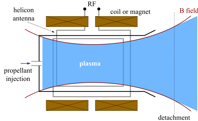
Figure 12. Schematic of a helicon plasma thruster.
