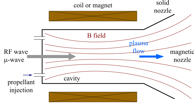
Figure 11. Outline of an electrodeless plasma thruster. The power is transferred to the gas from microwaves or RF waves. The plasma expands through either a solid nozzle or a magnetic nozzle. No neutralizer is required.
