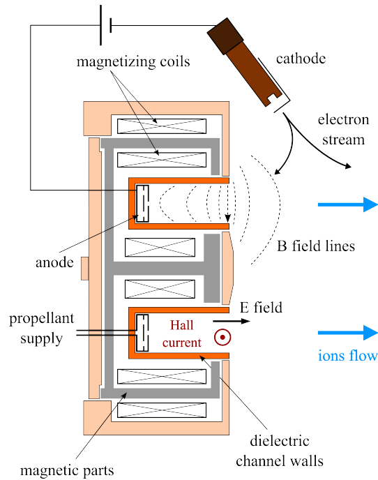
Figure 6. Schematic of a conventional annular Hall thruster with magnetizing coils and anode as fuel injector.
