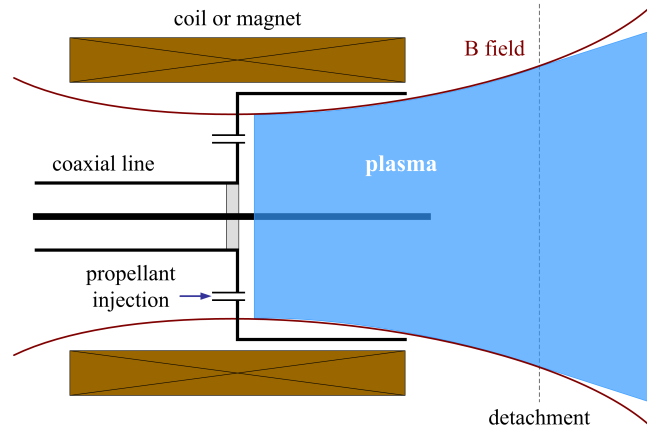
Figure 13. Schematic of the coaxial ECR plasma thruster [174].
