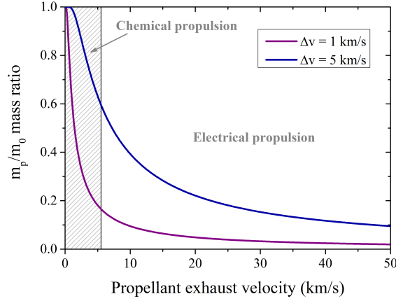
Figure 1. Ratio of the propellant mass to the initial mass as a function of the exhaust velocity v_e for two values of the velocity increment \Delta v . The dashed area corresponds to the domain of chemical propulsion with v_e below 5.5 km/s.
