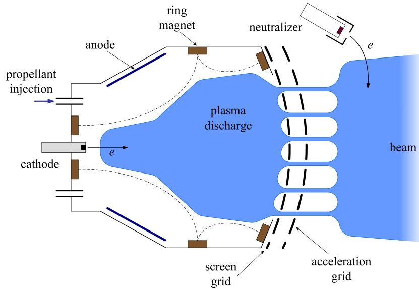
Figure 4. Schematic diagram of a DC electron bombardment gridded ion engine with 2 grids. A GIE is composed of three main elements: the ion source (DC, RF, \mu -wave), the acceleration stage with grids and the neutralizer.
