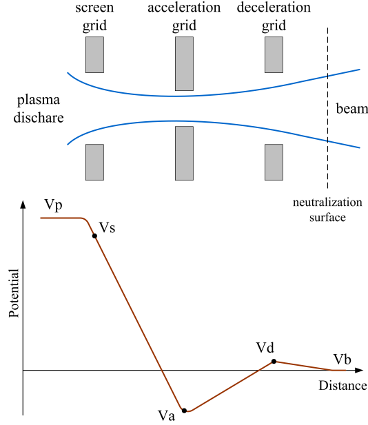
Figure 5. Schematic of a 3-grid system in an ion engine with the corresponding potential profile along the aperture axis.
