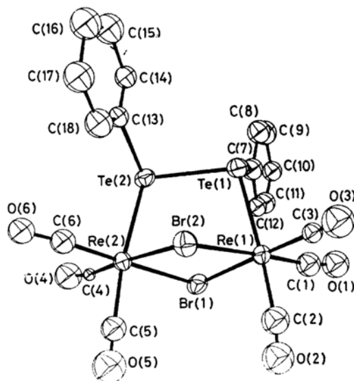
FIGURE 1 View of the molecule showing the folding along the Br...Br vector and the numbering system employed in the crystallographic study
