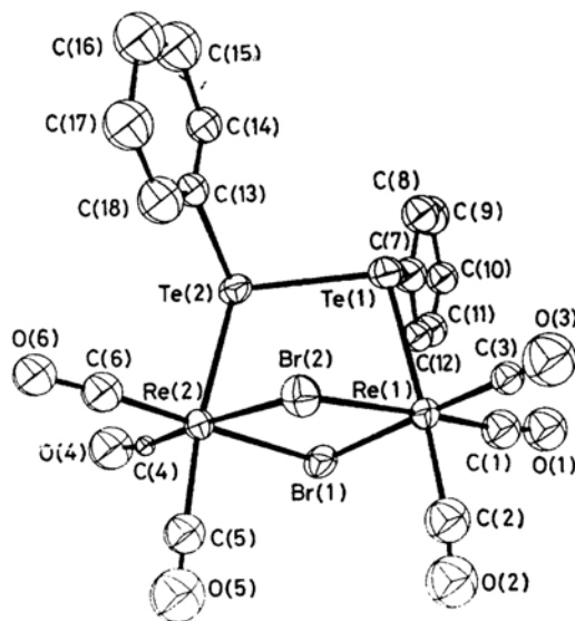
FIGURE 1 View of the molecule showing the folding along the Br...Br vector and the numbering system employed in the crystallographic study
