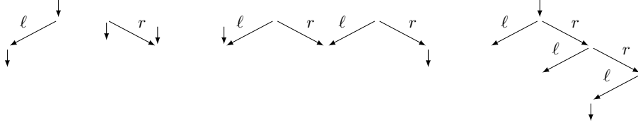
■ Figure 1 Munn bi-rooted trees of the elements of \mathcal{I}(\{\ell, r\}) : \ell , \bar{r} , \bar{\ell}r\bar{\ell} , and (\bar{\ell}r)^2\ell .
