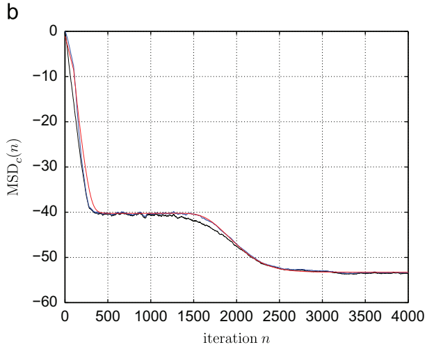
Fig. 3. Monte Carlo simulations averaged over 50 realizations for g_2[\xi(n)] with \sigma_o^2 = 10^{-4} , \delta = 0.1 and \mu_1 = 1/34 . (a) Behavior of E[\lambda(n)] and E[\lambda_o(n)] . Black (top curve): E[\lambda_o(n)] (optimum). Blue (superimposed by the red curve): E[\lambda(n)] from (17). Red (bottom curve): theory using (28). (b) Behavior of MSD_e(n) . Black: MSD_e(n) for \lambda_o(n) . Blue (bottom curve): MSD_e(n) from simulations. Red (top curve): theory using (35). (For interpretation of the references to color in this figure legend, the reader is referred to the web version of this article.)
