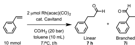
Scheme 5. Rhodium-catalyzed styrene hydroformylation
