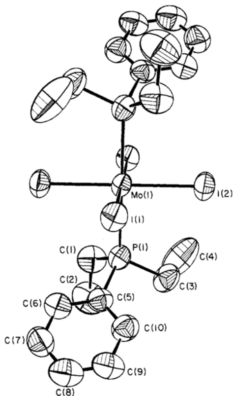
Figure 2. ORTEP view of one of the two crystallographically independent anions of compound 3.
