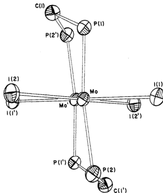
Figure 2. Central portion of the \text{Mo}_2\text{I}_4(\text{dppm})_2 molecule viewed along a direction close to the \text{Mo}-\text{Mo}' axis.
