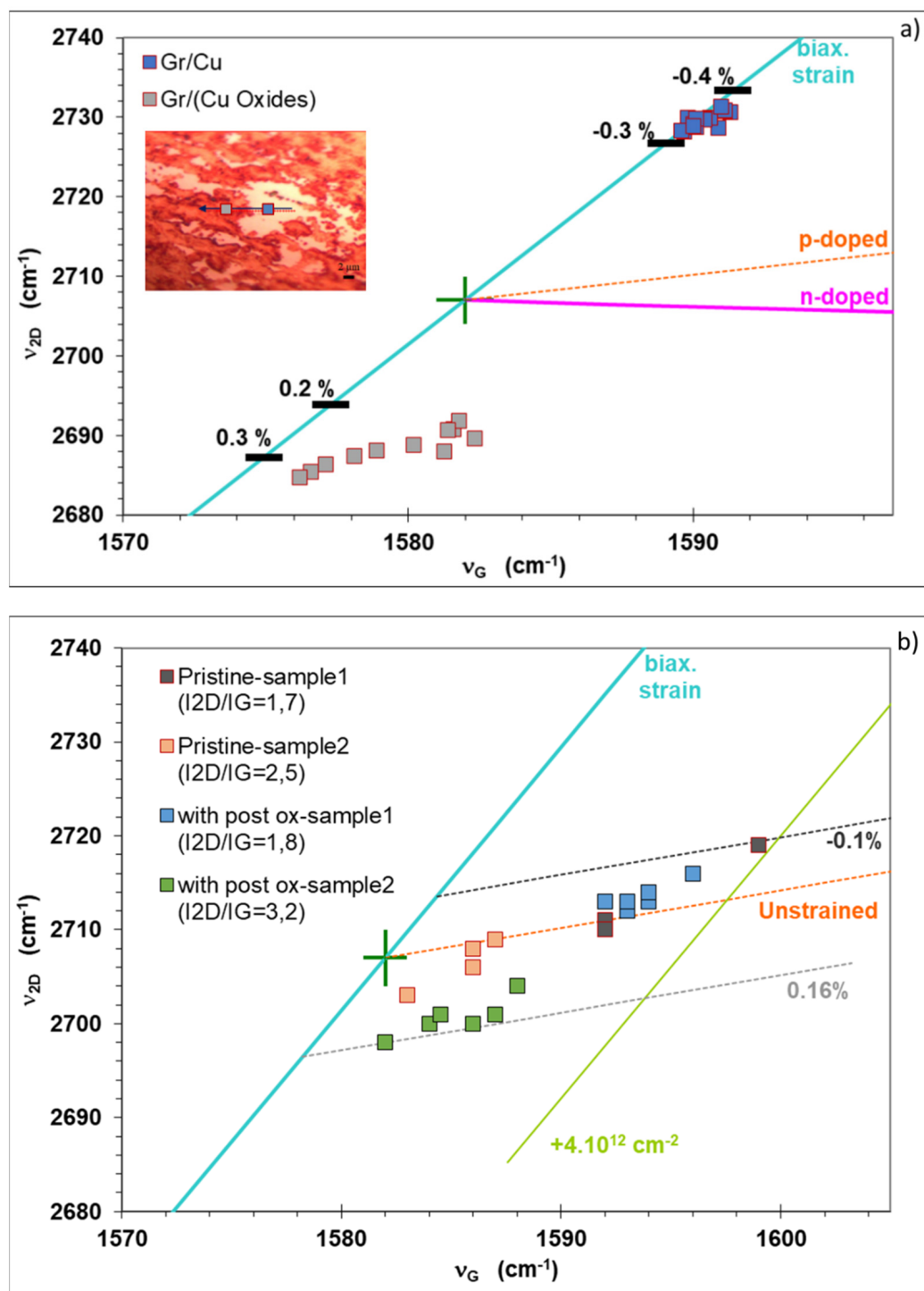
Figure 6. Correlation between the frequencies of the G and 2D Raman peaks of graphene ( \nu_G , \nu_{2D} ), from Raman spectra of 4 samples, with and without post-growth annealing. The green cross represents ( \nu_{G0} , \nu_{2D0} ) for undoped and unstrained graphene. The blue line (biax. strain) represents an estimation of ( \nu_G , \nu_{2D} ) for undoped graphene under biaxial strain, while the orange (respectively pink) dashed line corresponds to unstrained p-doped (n-doped) graphene. Horizontal black lines in panel a refer to the values of biaxial strain. (a) before transfer, (b) after transfer, the green line parallel to the blue one represents the ( \nu_G , \nu_{2D} ) strain dependency for a p-type doping of 4 \times 10^{12} \text{ cm}^{-2} .
