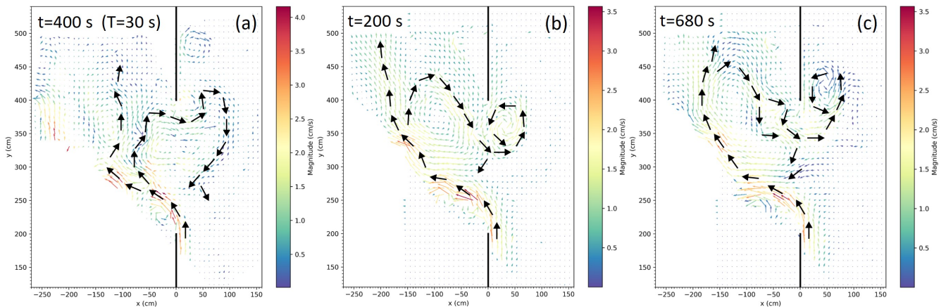
Figure 8. (a): Snapshot of the current velocity field (in cm\ s^{-1} ) at t = 400\ s for Q = 2 and T = 30\ s (cf. Supplementary Figures S3-S5). (b,c): same but for T = 60\ s at t = 200\ s and at t = 680\ s , respectively.
