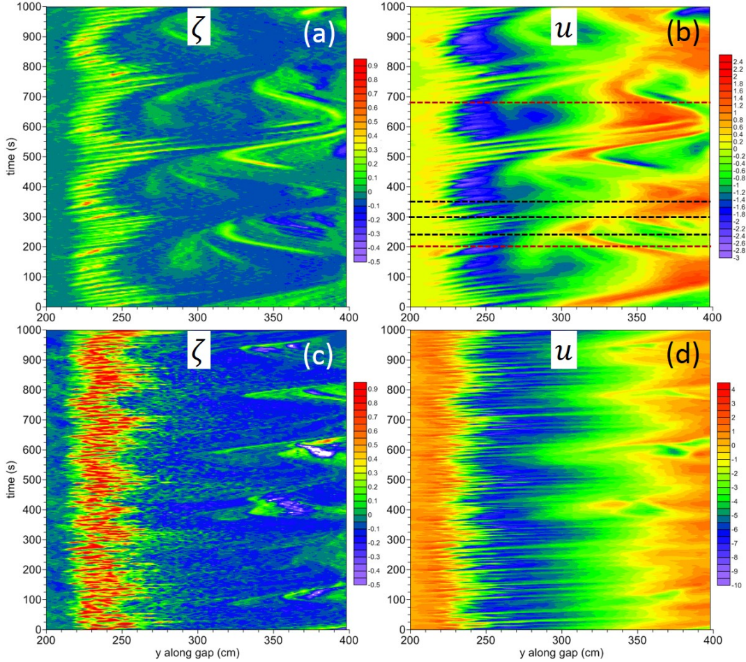
Figure 6. Hovmöller diagram of the relative vorticity \zeta (in s^{-1} ) –panel (a)– and current velocity u (in cm s^{-1} ) –panel (b)– for a rotation period T = 60 s and Q = 2 . Panels (c,d): same but with Q = 8 . The velocity profiles of u along the black dashed lines in panel (b) are shown in the Supplementary Figure S6 and the corresponding snapshots of the 2D \mathbf{u} –field are shown in Fig 7. The brown dashed lines in panel (b) correspond to the snapshots of Figs. 8(b,c).
