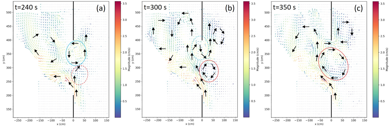
Figure 7. Snapshots of the current velocity field (in cm\ s^{-1} ) at t = 240\ s (a), t = 300\ s (b) and t = 350\ s (c) for Q = 2 and a rotation period T = 60\ s (see the black dots in Fig. 5(a), the u -field along black the dashed lines in Fig. 6(b) and Supplementary Figure S6 for the u -profiles along the gap).
