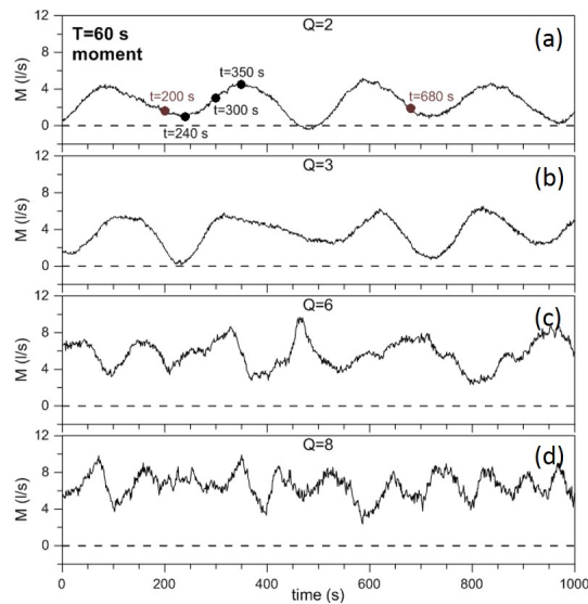
Figure 5. Time series of the moment M (in \text{litres s}^{-1} ) for different values of Q (2, 3, 6, 8) and for a rotation period T = 60 \text{ s} .
