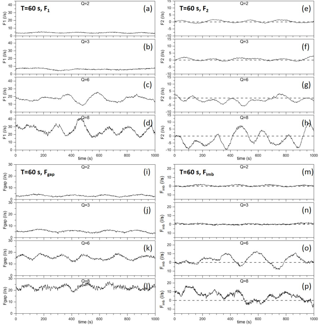
Figure 4. Time series of F_1 (a-d), F_2 (e-h), F_{gap} (i-l), F_{imb} (m-p) (units in litres\ s^{-1} ) for different values of Q (2, 3, 6, 8) and for a rotation period T = 60 s.
