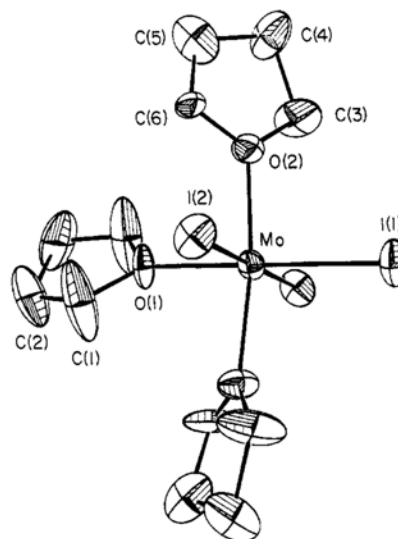
Figure 1. ORTEP view of MoI 3 (THF) 3 with the atomic numbering scheme employed.
