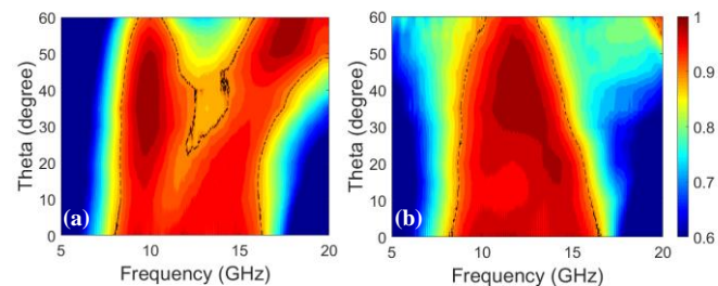
Fig. 5: Absorption level for \varphi=30^\circ : measurements in non-anechoic chamber for (a) vertical and (b) horizontal polarization. The dashed line in black corresponds to an absorptivity of 0.90.
