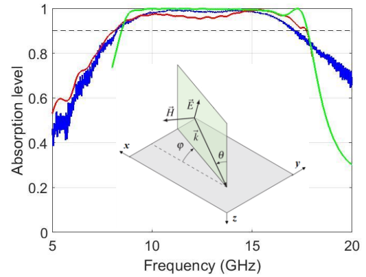
Fig. 3: Comparison between the simulation (green), and the measurements in anechoic chamber (red) and in non-anechoic chamber (blue) for \varphi = \theta = 0^\circ . The definition of \varphi (azimuth) and \theta (elevation incidence) angles are shown in the insert for the horizontal polarization (H-pol.) with the plane of incidence in green and the plane of the structure under test in grey. When \mathbf{E} and \mathbf{H} are inverted, vertical polarization (V-pol.) is considered.
