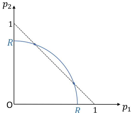
Figure 1. Schematic representation of the case n = 2 . The total probability constraint (6) is represented by the dashed straight line, while the entropy constraint (7) is represented by the blue quarter circle of radius R . Solutions are given by their intersections.
