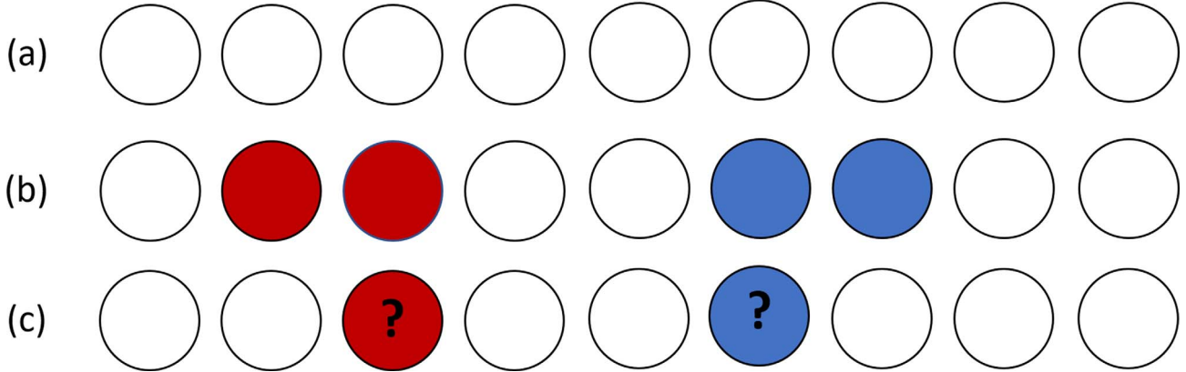
Figure 3. (a) Nine particles are drawn from a probability distribution p , corresponding to a pure state, but they are not yet observed. (b) We look at particles 2–3, which turn out to be both red, and then look at particles 6–7, which turn out to be both blue. (c) Had we drawn particles 3–6, we would have expected them to be of same color, but this is in contradiction with the “experiment” of row (b).
