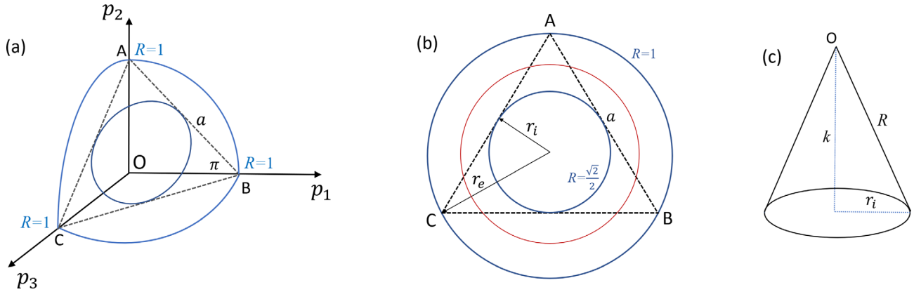
Figure 2. Schematic representation of the case n = 3 . (a) The solutions of equations (6) and (7) lie on the circle given by the intersection of the sphere of radius R (here represented for the pure state with R = 1 ) and the plane \pi passing through the points A, B and C. The dashed triangle ABC, lying on the plane \pi , has all sides equal to a = \sqrt{2} . The inner circle is inscribed into the triangle. (b) View of the plane \pi with the circumscribed and inscribed circles of radii r_e and r_i , which correspond, respectively, to values R = 1 and R = 1/\sqrt{2} . The thin red circle is an intermediate case where positive and negative probabilities coexist (the latter lie outside the triangle). (c) Circular cone with apex at the origin O and basis circle of radius r_i . The height k of the cone is the distance between the origin and the plane \pi .
