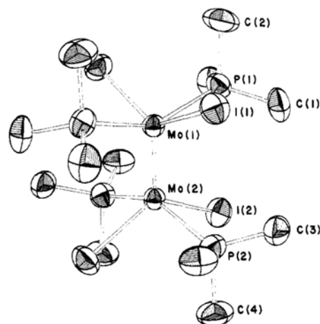
Figure 1. ORTEP view of the Mo 2 I 4 (PMe 3 ) 4 molecule.
