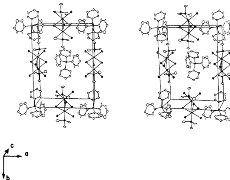
Figure 3. Stereoscopic view of the unit cell of compound 3.
