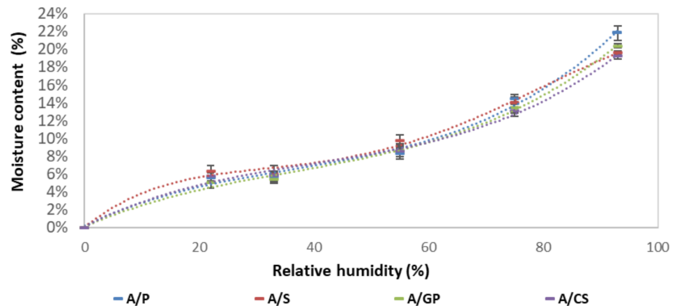
Figure 4. Sorption isotherms of the four composites.
