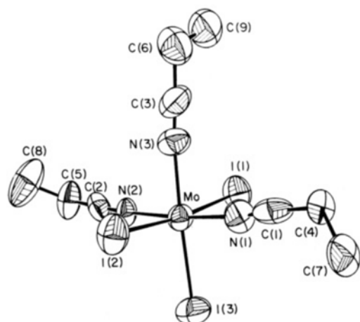
Figure 9. ORTEP view of compound 4.
