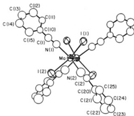
Figure 10. ORTEP view of compound 6.
