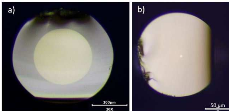
Fig. 12. Optical micrographs of different fibers cleaves: a) 170μm core fiber diameter obtained with the large-core preform resulting from the BIC method and b) small-core fiber (7μm core diameter) prepared through the RiT method
