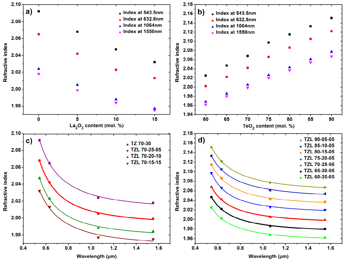
Fig. 7. Refractive index as a function of the \text{La}_2\text{O}_3 content variation (a) and at fixed \text{La}_2\text{O}_3 content (b). Wavelength-dependent refractive index with the Sellmeier equation for \text{La}_2\text{O}_3 content variation (c) and at fixed \text{La}_2\text{O}_3 content (d) ( in bold red and black, the two compositions chosen for optical fibers drawing )
