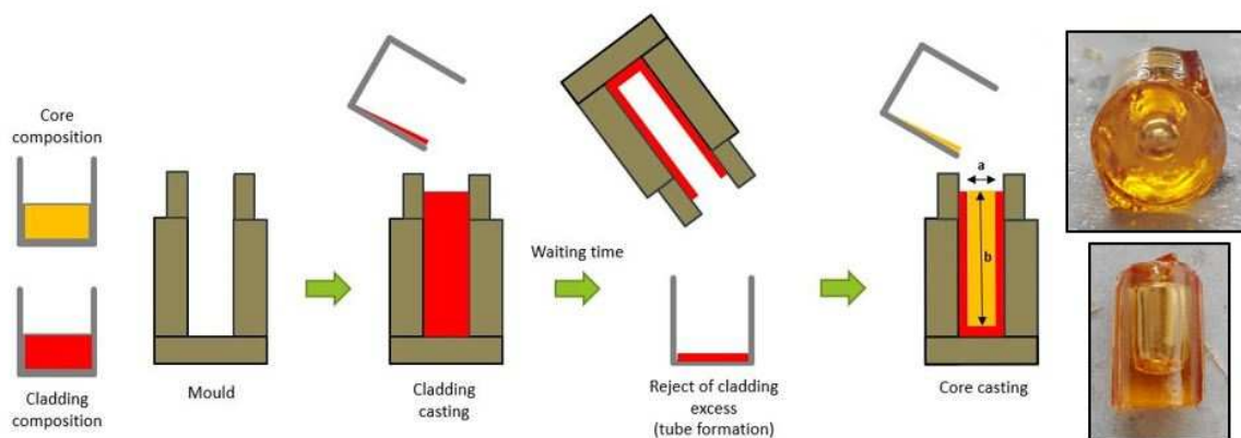
Fig. 1. Core-cladding preform preparation by Built-in-Casting technique
