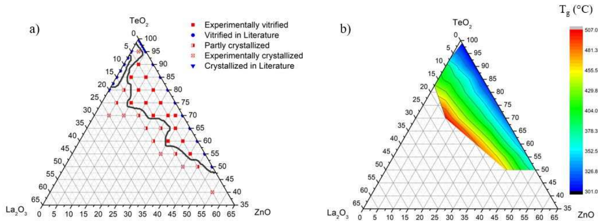
Fig. 2. a: TZL ternary diagram; b: composition influence on the glass transition temperature (Binaries coming from literature: TeO 2 -La 2 O 3 [20] and TeO 2 -ZnO [21])
