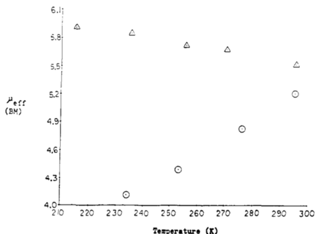
Figure 3. Temperature dependence of the effective magnetic moment for FeCl 3 (PR 3 ) 2 (R = Me, Cy): O, Me; \Delta , Cy. Measurements were done by NMR spectroscopy in toluene- d 8 . No correction for the diamagnetic contribution or for the solution density change with temperature was applied.
