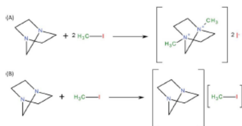
Fig. 2 (A) Formation of a non-volatile quaternary ammonium salt by an S_N2 mechanism between TEDA and CH_3I . (B) Secondary neutral complex formed between TEDA and CH_3I . 75
