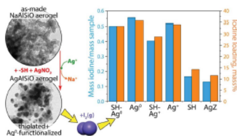
Fig. 9 Comparison of the iodine adsorption capacities of different silver-functionalized aerogels (SH-Ag 0 , Ag 0 , SH-Ag + , Ag + , and SH) with that of a silver-loaded mordenite (AgZ). 102 Reprinted with permission from B. J. Riley, J. O. Kroll, J. A. Peterson, J. Matyáš, M. J. Olszta, X. Li and J. D. Vienna, ACS Applied Materials & Interfaces , 2017, 9, 32907–32919. Copyright 2017 American Chemical Society.
