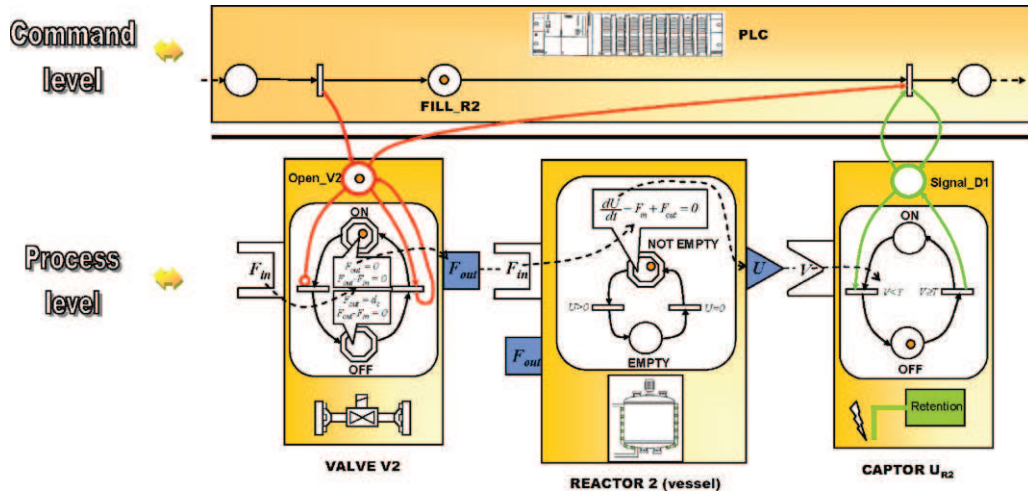
Fig. 16. Interaction between process and command level.
