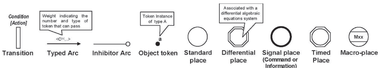
Fig. 14. Semantic elements of ODPN formalism.
