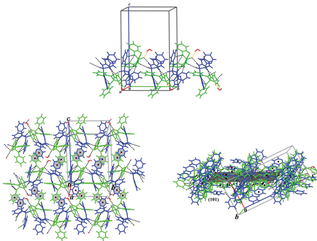
Fig. 7 Up: partial view of one-dimensional (1D) chain formed via N–H···O and N–H···N (black dash lines), and O–H···O (orange dash lines) hydrogen bond interactions along the b axis in the crystal structure of 3 . Down: the 1D chains are connected via \pi ··· \pi stacking interaction (red dash lines) building a two-dimensional (2D) molecular assembly parallel to the (101) plane showed in two views. The symmetrically independent molecules are specified by different colors.
