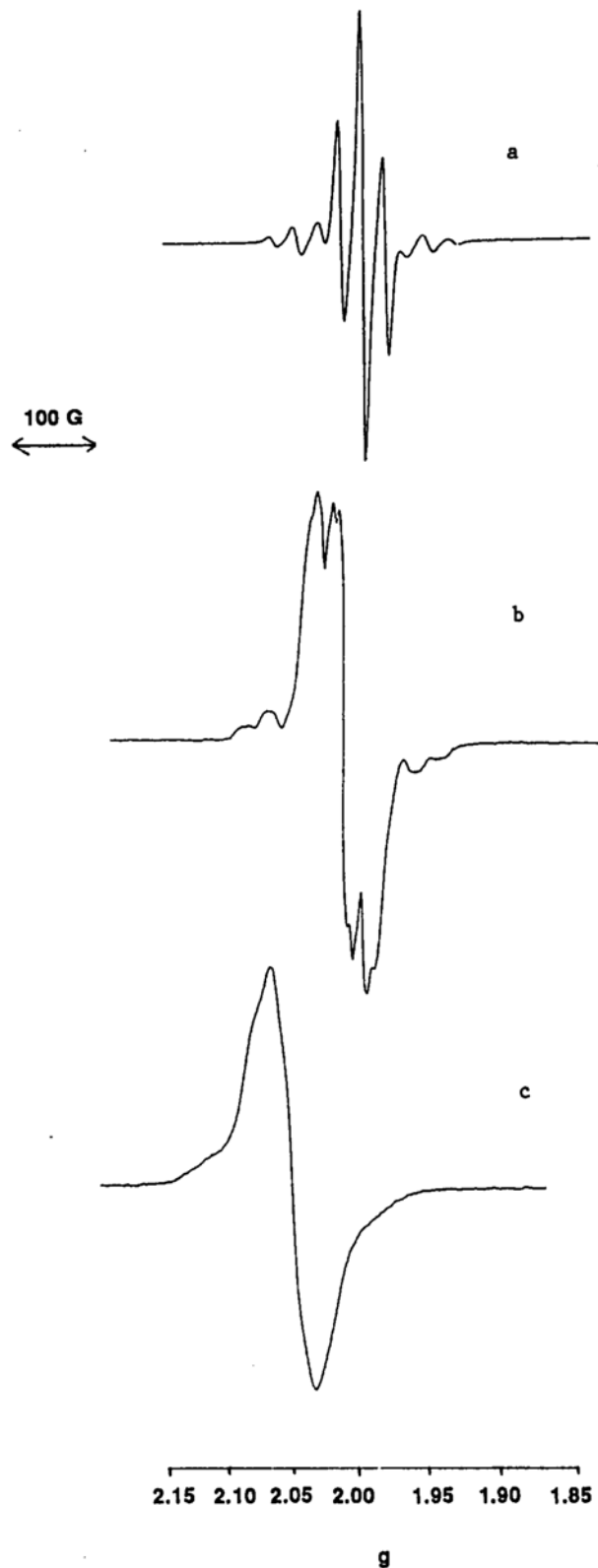
Figure 1. EPR spectra of compounds MoCpX 2 (dppe) at room temperature with CH 2 Cl 2 as solvent: (a) X = Cl; (b) X = Br; (c) X = I.
