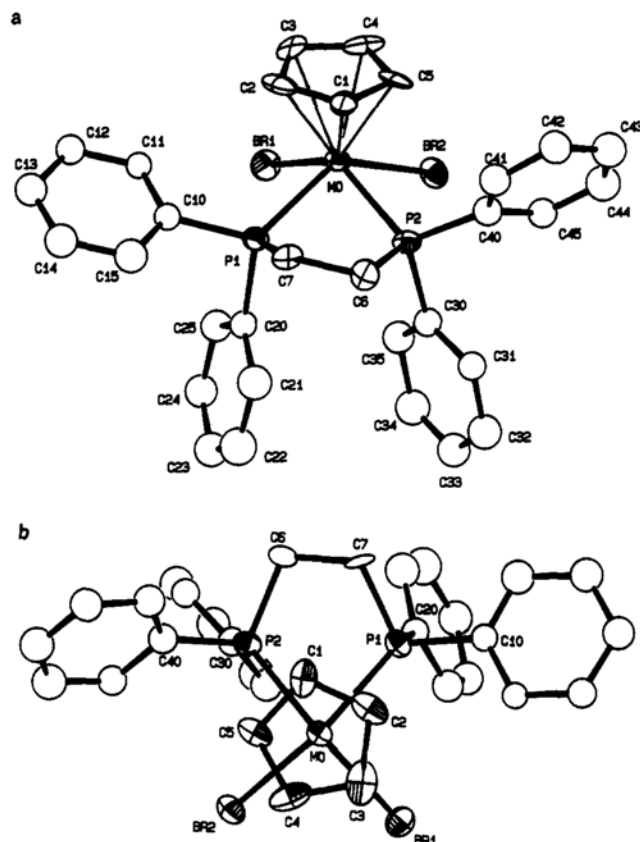
Figure 2. (a) ORTEP view of the \text{MoCpBr}_2(\text{dppe}) molecule, showing the atomic numbering scheme employed. Hydrogen atoms have been omitted for clarity. Thermal ellipsoids are at the 40% probability level. (b) View of the \text{MoCpBr}_2(\text{dppe}) molecule along an axis approximately perpendicular to the Cp ring plane. The ORTEP plot files were modified with the program PLOTMD 32 for label position optimization.
