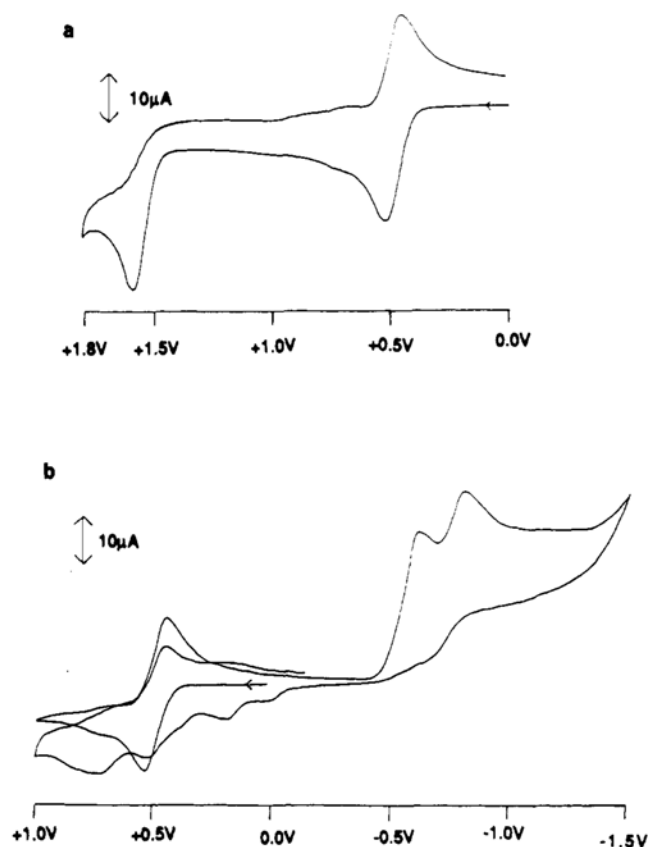
Figure 3. Cyclic voltammograms of MoCpBr 2 (dppe) in CH 2 Cl 2 (scan speed = 200 mV·s −1 ): (a) showing the two oxidation processes; (b) showing the reduction processes and the effect of these on the quasi-reversible first oxidation process.
