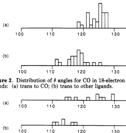
Figure 3. Distribution of \theta angles for phosphine and phosphite ligands in 18-electron compounds: (a) trans to CO or other phosphine; (b) trans to non- \pi -acidic ligands.
