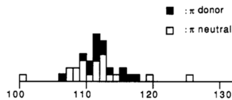
Figure 1. Distribution of \theta angles for \pi -neutral and \pi -donor ligands in 18-electron compounds.
