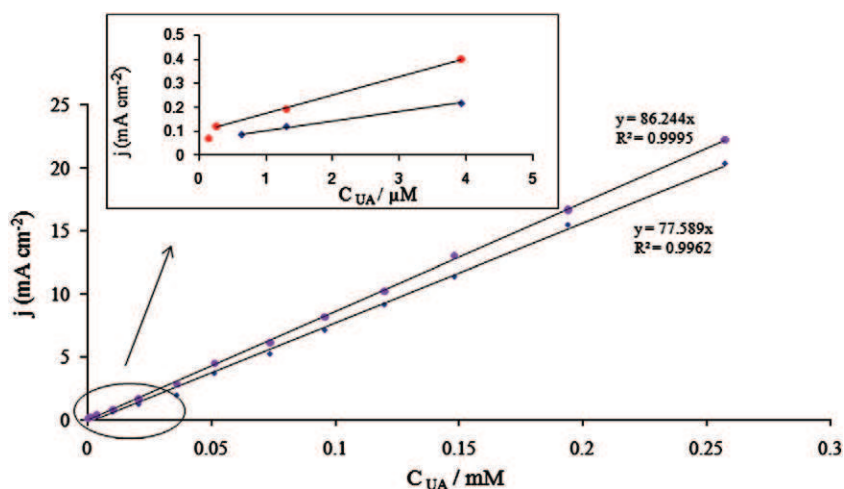
Fig. 2. Calibration curve of the \mu\text{Au} -PEDOT to UA assay without (♦) or with AA 1 mM (●) in the calibrating solutions. Detection potential: 0.24 V. The inset shows the curve for low UA concentrations.
