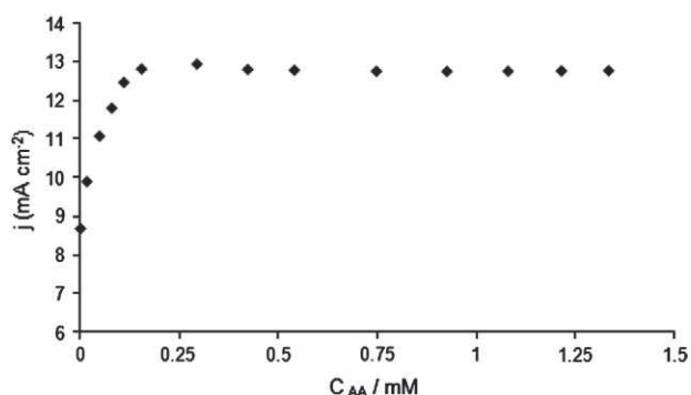
Fig. 3. Influence of the AA concentration on the amperometric response of the \mu\text{Au-PEDOT} to UA 100 \mu\text{M} detection potential: 0.24 \text{ V} .
