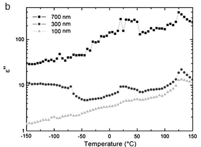
Fig. 8. Temperature dependence of (a) \epsilon' and (b) \epsilon'' ( f = 1 kHz) of BaTiO 3 ceramics sintered by Spark Plasma Sintering from nanoparticles of (■) 700 nm, (●) 300 nm, (▲) 100 nm.
