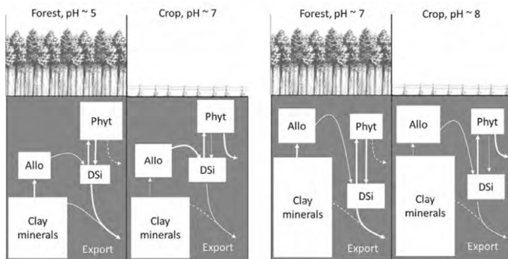
Fig. 8. Adaptation of the Struyf et al. (2010) conceptual model for the impact of land use change from mature forests to long-term cultivated areas on the main pools that control soluble Si in soils developed on loess (left-hand side) and calcareous soils (right-hand side). Boxes represent the main Si pools with the size of the boxes representing the relative size of the stock. Arrows represent fluxes with a thickness depending on their relative importance. Dashed arrows represent irrelevant fluxes. Ph, Si in phytoliths; DSi, soluble Si estimated by \text{Si}_{\text{CaCl}_2} ; Allo, Si in allophanes.
