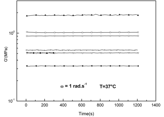
Fig. 5 – Storage modulus G'(t, 1 \text{ rad s}^{-1}, 37 \text{ °C}) as a function of time at the angular frequency of 1 rad s -1 , at the temperature of 37 °C for all the soft liner samples: (□) plasticized PMMA, (◄) plasticized PEMA, (▲) PI, (◇) PSi HTV, (+) PSi RTVg, (■) PSi RTVp, (∇) PSi RTVu.
