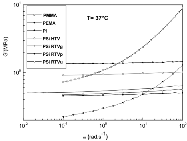
Fig. 3 – Storage modulus G'(\omega) as a function of frequency taken at the mucosa temperature of 37 °C for all the soft liner samples: (□) plasticized PMMA, (◄) plasticized PEMA, (▲) PI, (◇) PSi HTV, (+) PSi RTVg, (■) PSi RTVp, (∇) PSi RTVu.
