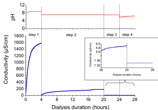
Fig. 5. Evolution of the conductivity and pH of the dialysis medium vs. time for apatite colloid doped with 1.5 mol.% Eu (relative to Ca).
