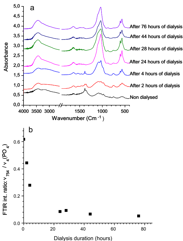
Fig. 2. Evolution of (a) FTIR spectra vs. dialysis time for Eu-free apatite colloid and (b) FTIR intensity ratio \nu_{754} / \nu_4(\text{PO}_4) .
