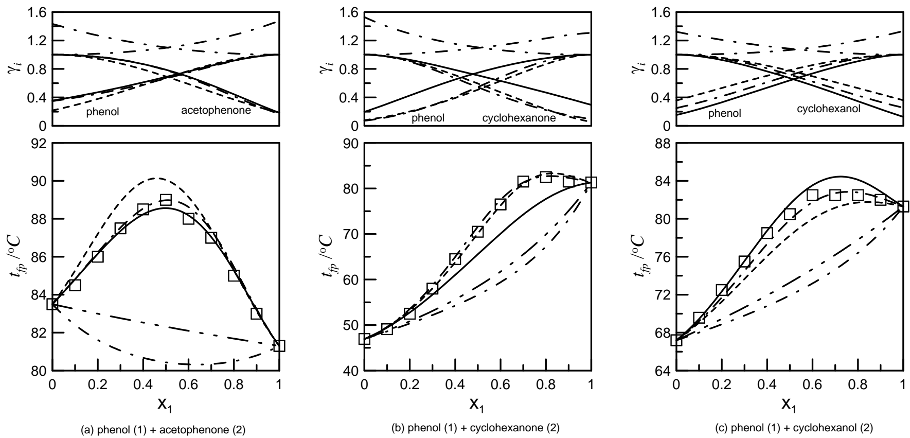
Figure 7. Comparison of predicted flash point and experimental data for maximum flash point solutions. \square , experimental data; —, original UNIFAC; - - - , UNIFAC Dortmund 93; - · - , UNIFAC Lyngby; - · · - , NRTL; - - - - , ideal solution.
