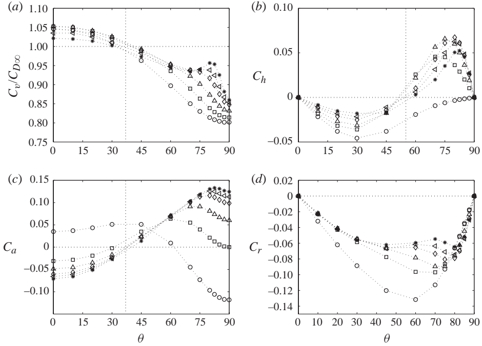
FIGURE 9. (a–d) Effect of the Reynolds number on the coefficients C_v/C_{D\infty} , C_h , C_a and C_r for S=3 . Symbols: *, Re = 500 ; <, Re = 300 ; \diamond , Re = 200 ; \triangle , Re = 100 ; \square , Re = 50 ; \circ , Re = 20 . Vertical dashed lines show \theta_v = 37^\circ , \theta_h = 55^\circ and \theta_a = 37^\circ , respectively.
