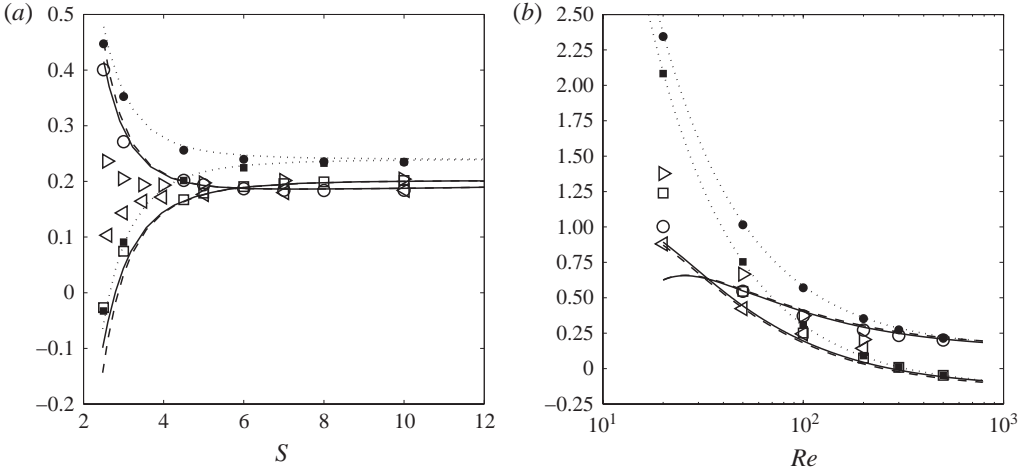
FIGURE 5. Evolution of the drag coefficient for two bubbles moving in line ( \theta = 90^\circ ): (a) for Re = 200 and (b) for S = 3 . Lines and symbols: \cdots , potential solution (4.10)–(4.11); --- , relations (1.3)–(1.4) from Harper (1997); - , relations (4.12)–(4.13). Numerical simulations: \circ , C_{D1} ; \square , C_{D2} ; \bullet , C_{D1_{pot}} ; \blacksquare , C_{D2_{pot}} (this study); \triangleleft , C_{D1} and \triangleright , C_{D2} (Yuan & Prosperetti 1994; from their figure 2).
