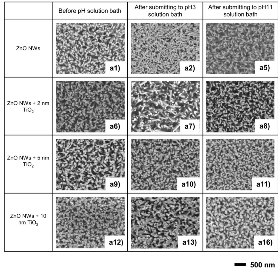
Figure 2. SEM images of the effect of TiO 2 coating thickness on ZnO NWs in strong acid/alkaline aqueous solutions.
