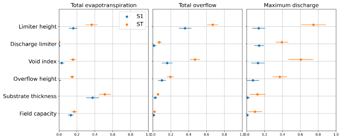
Figure 1. Results of the 6-parameter sensitivity analysis (case 1) depending on the indicator used (total evapotranspiration, total overflow, maximum discharge). S1 is the first order Sobol indices and ST the total effect indices.
