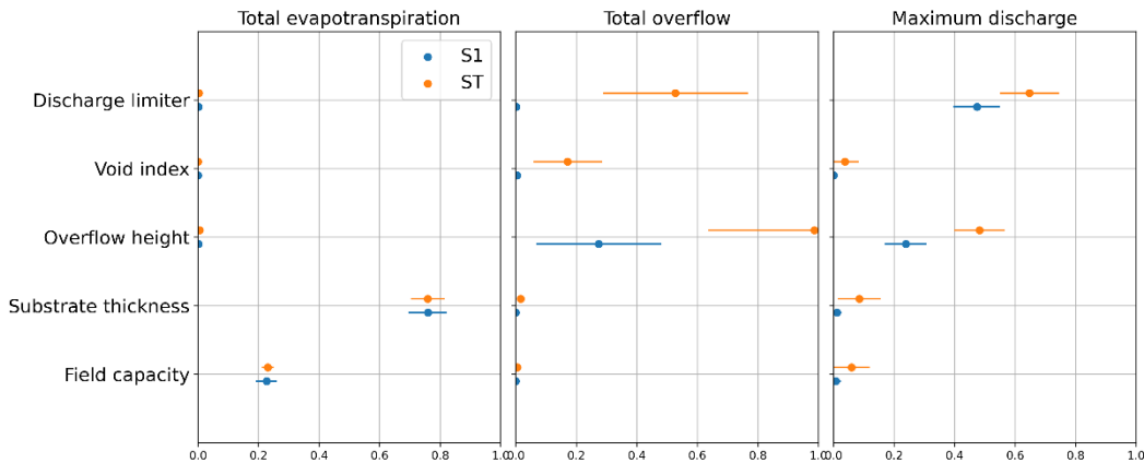
Figure 2. Results of the 5-parameters sensitivity analysis (case 2) depending on the indicator used (total evapotranspiration, total overflow, maximum discharge)
