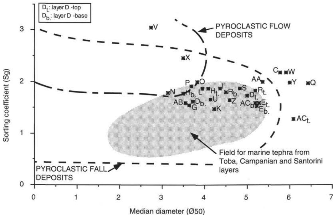
Figure 3. Median grain size ( \phi_{50} ) vs. sorting coefficient ( S_g ) for deep-sea tephra layers in Hole 907A. Fields of pyroclastic flow deposits and pyroclastic fall deposits are from Walker (1971). Marine tephra field from Toba, Campanian, and Santorini layers is from Ninkovich et al. (1978).
