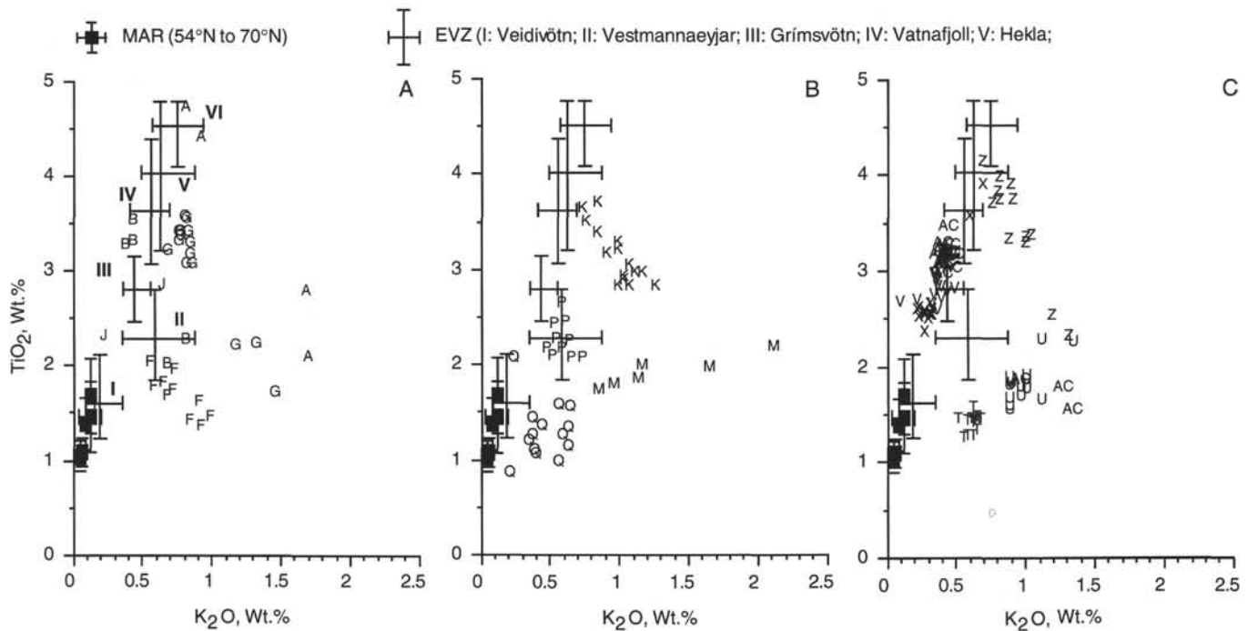
Figure 8. \text{TiO}_2/\text{K}_2\text{O} plots for basaltic and basaltic andesitic glasses from (A) Pleistocene, (B) late Pliocene, and (C) early Pliocene tephra in Hole 907A. All analyses have been normalized to a total of 100%. Fields for the Eastern Volcanic Zone (EVZ) in Iceland after Jakobsson (1979b). Fields for the Mid-Atlantic Ridge (MAR) after Sigurdsson (1981).
