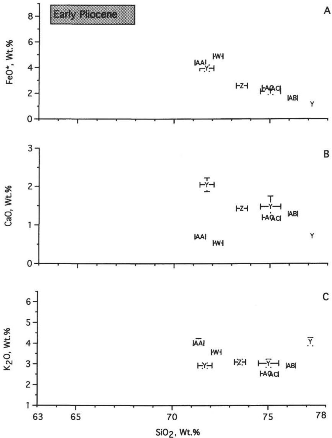
Figure 11. Fields of rhyolitic glasses from early Pliocene tephra in Hole 907A in (A) \text{FeO}^*/\text{SiO}_2 , (B) \text{CaO}/\text{SiO}_2 , and (C) \text{K}_2\text{O}/\text{SiO}_2 diagrams. All analyses have been normalized to a total of 100%. Crosses are mean and standard deviation.
