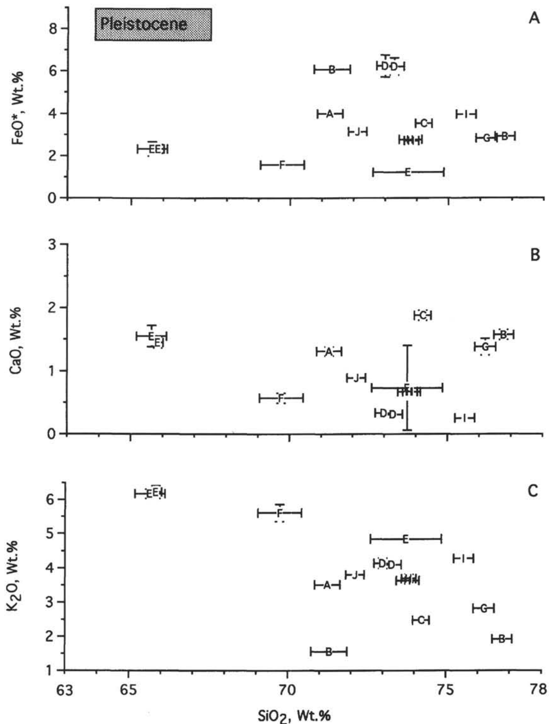
Figure 9. Fields of trachytic and rhyolitic glasses from Pleistocene tephra in Hole 907A in (A) FeO*/SiO 2 , (B) CaO/SiO 2 , and (C) K 2 O/SiO 2 diagrams. All analyses have been normalized to a total of 100%. Crosses are mean and standard deviation.
