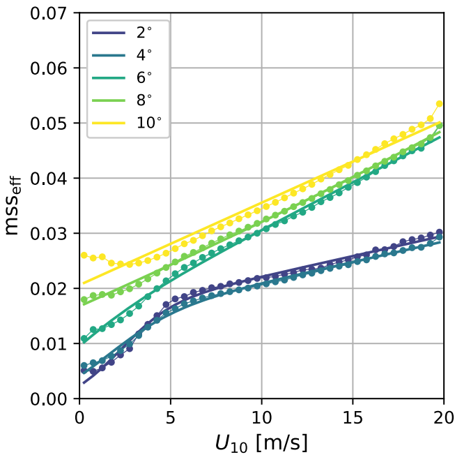
Figure 7. m_{SS_{eff}} parameter estimated from least squares fitting of average Normalized Radar Cross-Section profiles (Equation 15) (dots) and parameterization (Equation 29) (solid line) for SWIM off-nadir beams.
