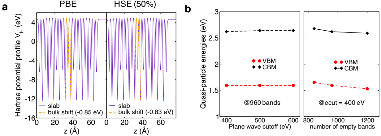
FIG. 5: Theoretical methods for the absolute energy level alignment considering CsPbI 3 bulk and slabs. a Comparison of the Hartree potential shifts computed at the PBE+SOC and HSE06+SOC ( \alpha = 50\% ) levels of theory using VASP. The figures are obtained using CsPbI 3 slab. \Delta V_H is similar in both cases which partly justifies the use of \Delta V_H from the DFT level for the absolute valence energy level alignment using the quasi-particle energies from G0W0 approximation. b Convergence of the G0W0 quasi-particle energies at VB/CB of bulk CsPbI 3 with respect to the response function cutoff and the number of empty bands. Note that, by default, VASP uses 2/3 of the plane wave cutoff for the energy cutoff of the response function.
