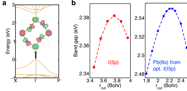
FIG. 1: Optimization of DFT-1/2 r_{cut} values of I and Pb using the tetragonal MA*PbI 3 . a Band structure of MA*PbI 3 in the tetragonal phase. The wavefunction, without SOC, at the VBM occurring at the \Gamma point is also shown in the figure. b Optimizing r_{cut} for (left) the pseudopotential of I by removing 1/2 e^- from its 5p states (right) Pb atom with the removal of 1/2e^- from its 6s states using the optimized I(5p) atom from the left. Here the optimal r_{cut} are \sim 3.76 Bohr and \sim 2.20 Bohr for I and Pb, respectively. Note that spin-orbit coupling (SOC) effect is not taken into account here since it is not necessary for the optimization of r_{cut} .
