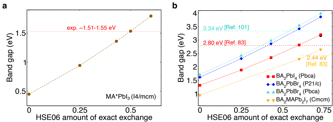
FIG. 4: Impact of the amount of HSE06 exact exchange \alpha on band gap prediction in halide perovskites. a Variation of the band gap of the room temperature 3D MA*PbI 3 MHP with the amount of exact exchange \alpha . b Variation of the band gap of different 2D MHP with the amount of HSE06 exact exchange \alpha . Horizontal dashed lines correspond to the experimentally reported electronic band gap values for the compounds of the same color.
