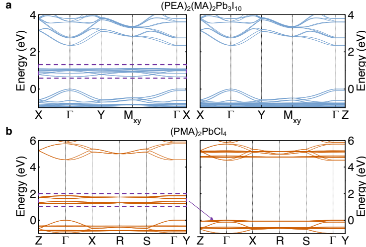
FIG. 3: Evidencing the necessity to correct molecular states in some 2D MHP. a Band structure of (\text{PEA})_2(\text{MA})_2\text{Pb}_3\text{I}_{10} structure using xs-DFT-1/2 (left) without DFT-1/2 correction on molecular states and (right) with DFT-1/2 correction on molecular states. b Band structure of (\text{PMA})_2\text{PbCl}_4 structure using xs-DFT-1/2 (left) without DFT-1/2 correction on molecular states and (right) with DFT-1/2 correction on molecular states. The molecular states are shown in the dashed rectangular boxes.
