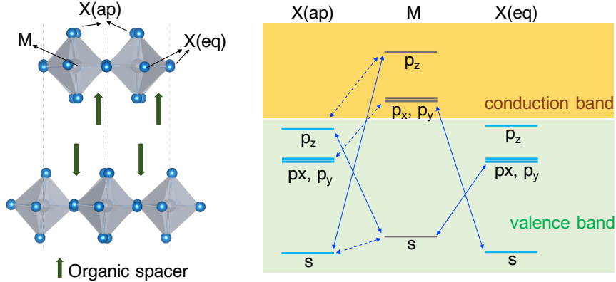
FIG. 2: Symmetry analysis of 2D MHP 2,85 . (left) An example of a 2D MHP structure showing the apical and equatorial halide X atoms along with the central metal M atom. (right) Electronic coupling between X and M states expected from the symmetry analysis of 2D MHP.
