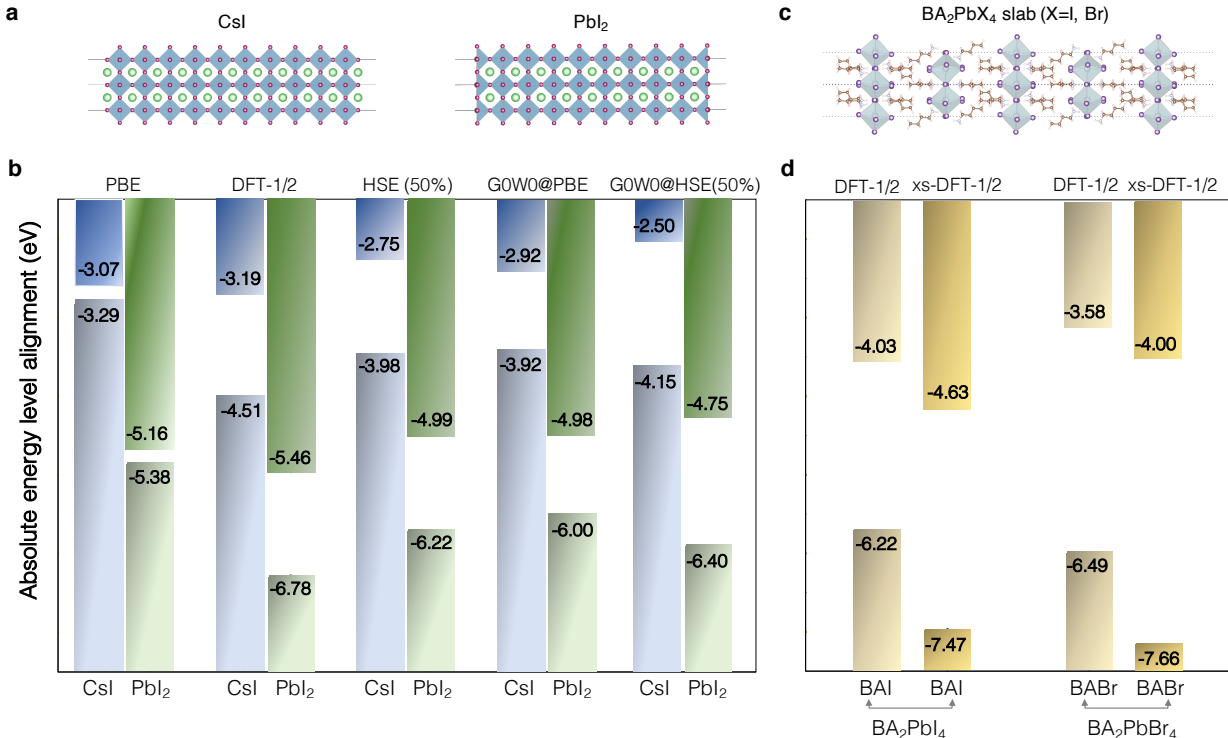
FIG. 6: Slab structures and computation of the absolute valence energy levels of MHP at different levels of theory. a CsPbI 3 slabs with CsI and PbI 2 -terminations used for the computation of the absolute valence energy levels. b Comparison of the absolute valence energy level of pseudo-cubic CsPbI 3 with different terminations at different levels of theory. Here, PBE results are obtained using VASP to be consistent with HSE and G0W0@PBE c Slab structures used to compute E_v^{abs} for BA 2 PbI 4 and BA 2 PbBr 4 . d Comparison of the absolute valence energy levels of BA 2 PbX 4 (X = I, Br) with BAX-termination at DFT-1/2 and xs-DFT-1/2 corrections.
