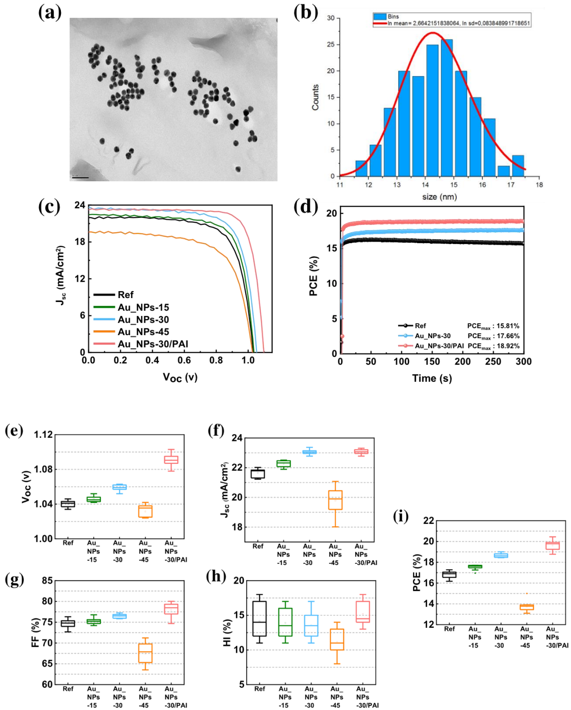
Figure 1. (a) TEM view images of gold nanoparticles. (b) Statistical grain size analysis. (c) J - V reverse curves. (d) Maximum power point (MPP) tracking and best-stabilized efficiency. (e-i) Statistical analysis of the optimized PSCs J - V curve parameters and PCE.
