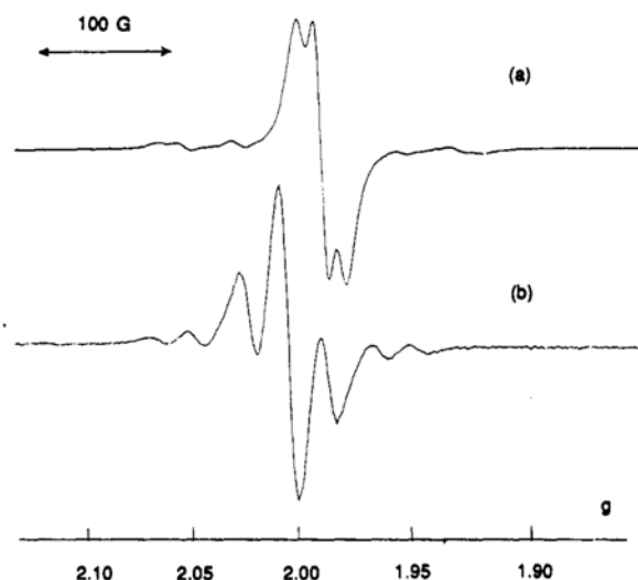
Figure 1. EPR spectrum of \text{CpMoCl}_2(\text{PMe}_3)_2 : (a) solvent = THF, room temperature; (b) after reaction with 2 equiv of \text{MeLi} , T = 270 K.
